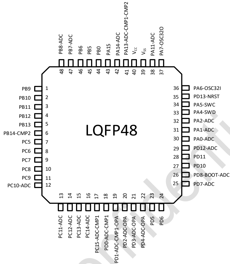
Figure 3-2 LQFP48 Pinout2 PY32L090C2xT7 (Top view)
